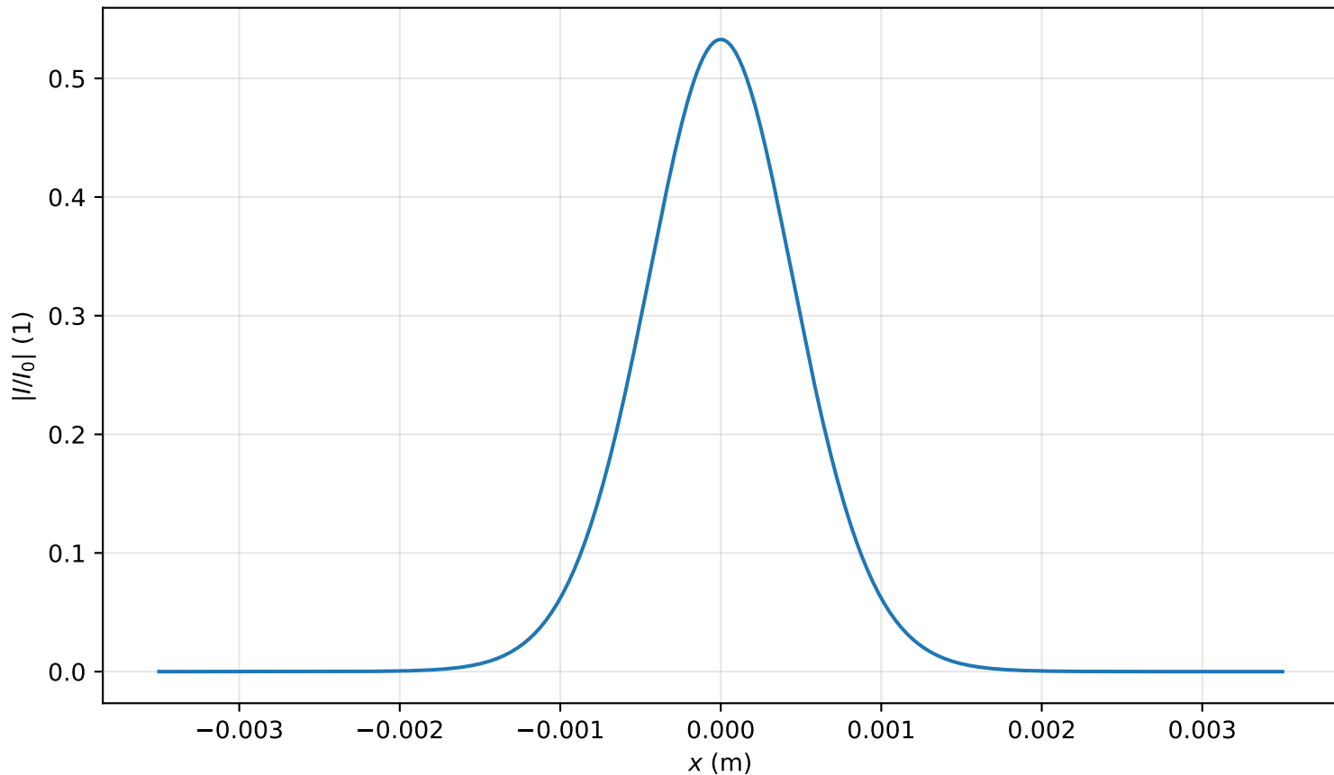
Intensity profile I(x, y = 0, z = 2.468m)/I_0 , P_{in}=0.3P_{cr} , artificial time
